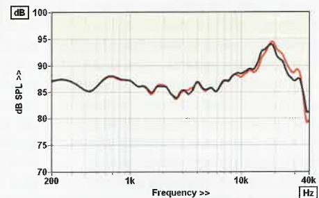
ABOVE: Forward response indicates a depressed presence band relative to a rising (high) treble
