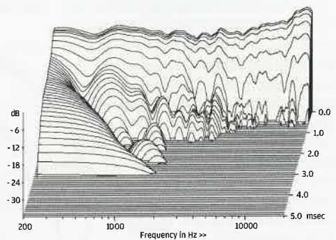
ABOVE: Cabinet modes are mild but the driver resonance at ~4kHz also appears in the freq. resp.
